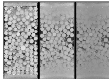
Evolution of the structure of a sample (pellets + powder pellets) following an imbibition (by the lower and upper faces) to: • t = 0 day (left) • t = 4 days (centre) • t = 8 days (right) (Molinero, 2017)
